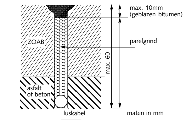
..... Figuur 5.6 Drainage in ZOAB
