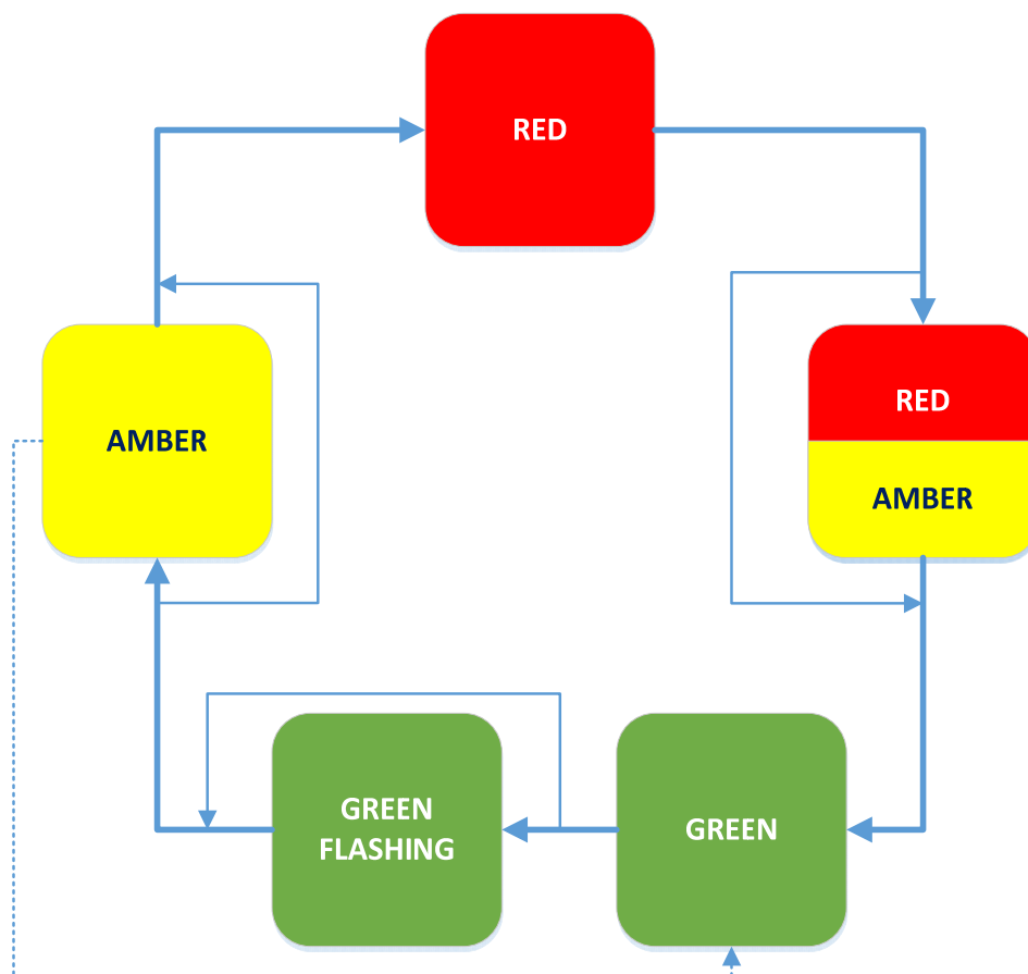
Figure 5 Signal group control-state transitions (Control)
