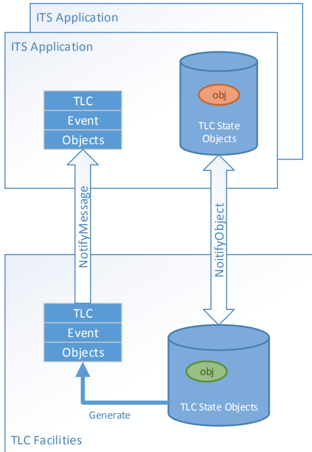
Figure 8 Object exchange
