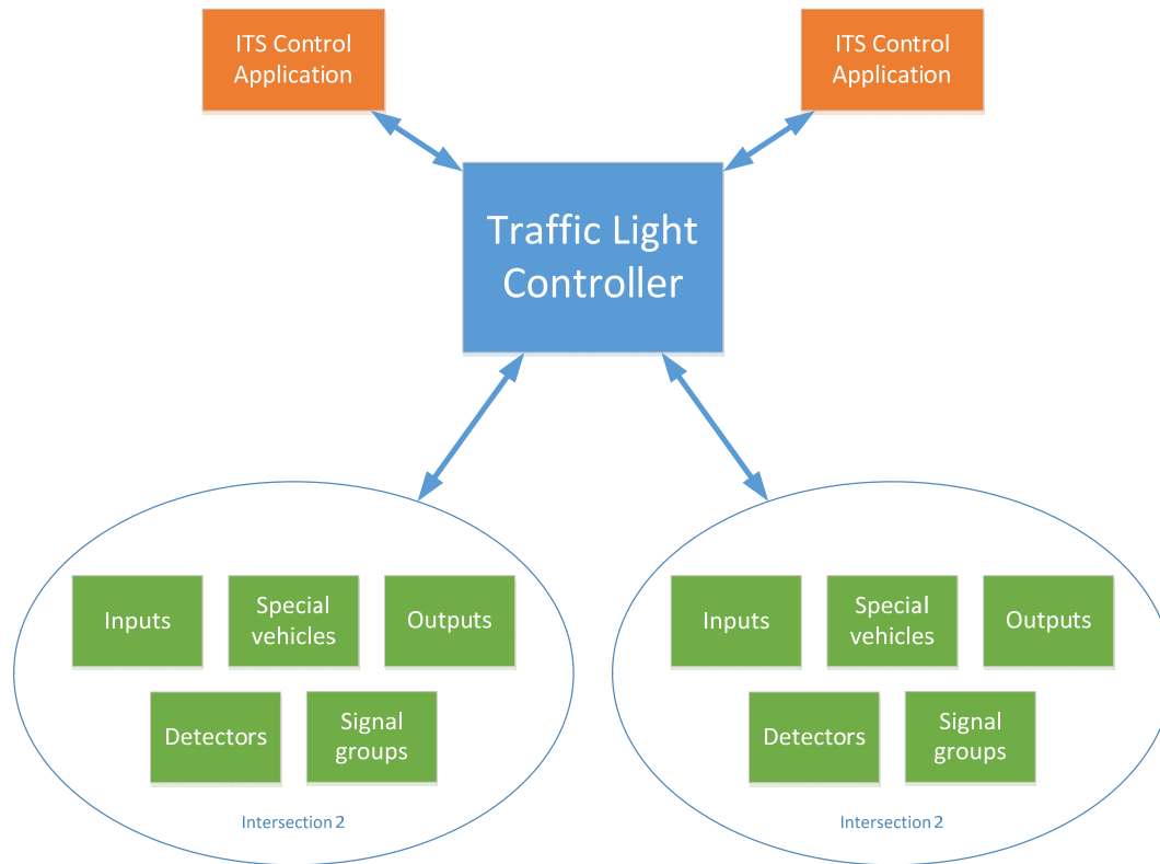
Figure 3 Multiple intersections
