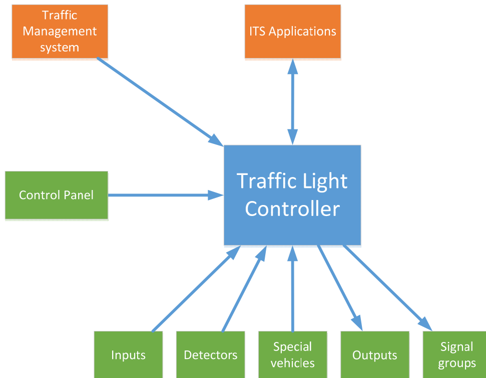
Figure 2 TLC context
