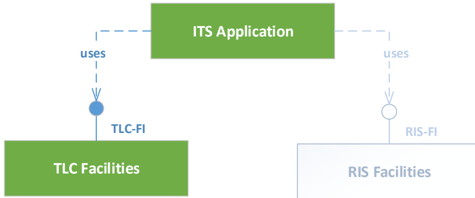
Figure 1 TLC-FI in System overview
