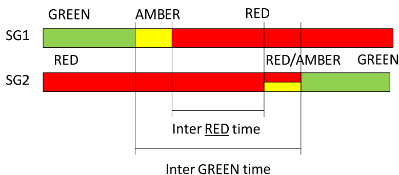
Figure 6 Clearance timing
