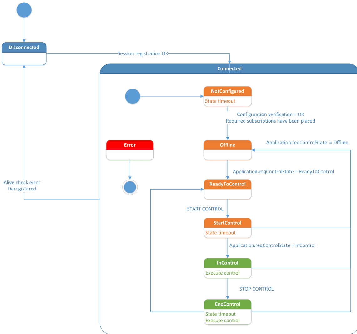
Figure 7 ITS-CLA – Control State transitions
